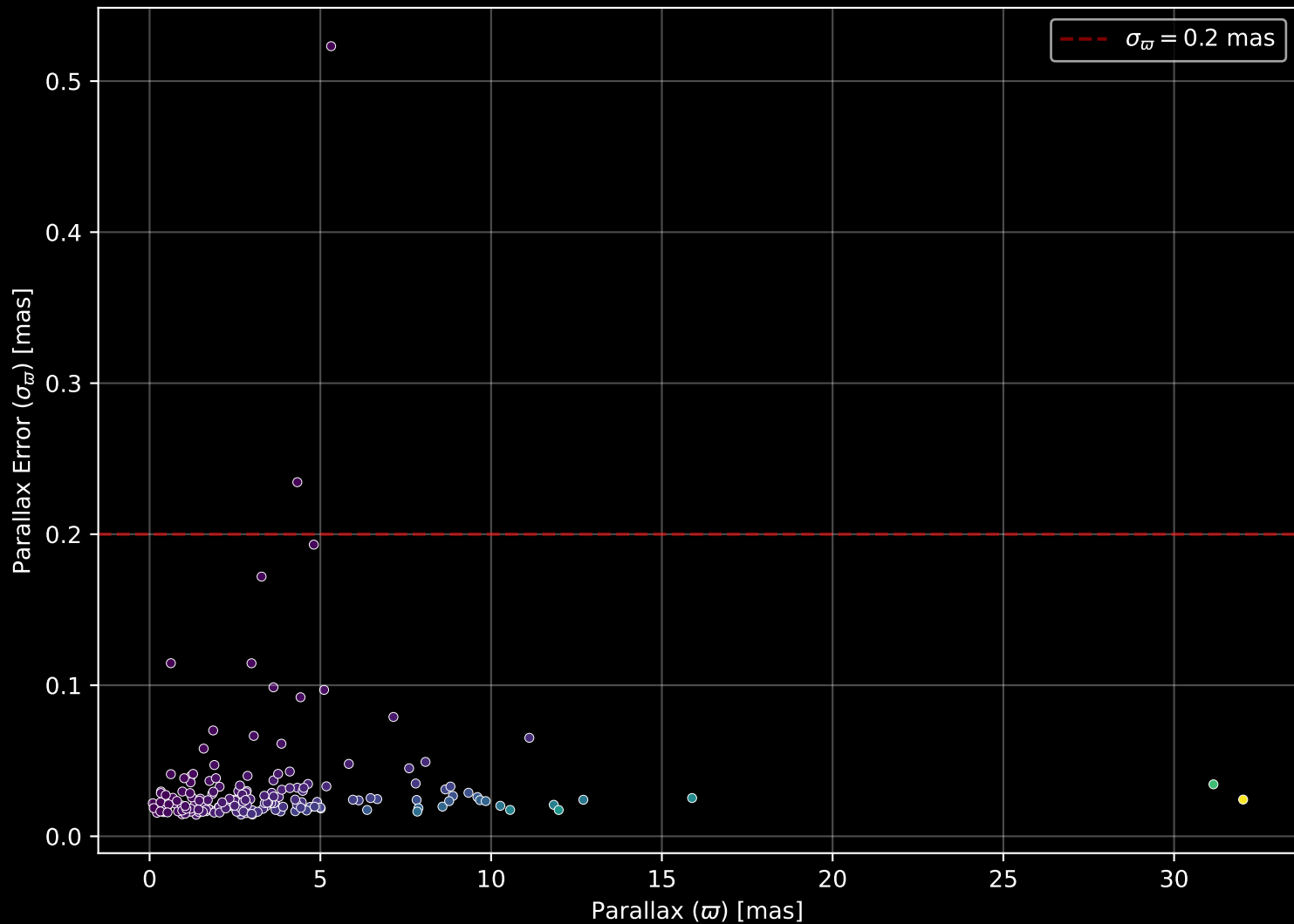
APOGEE DR17 Field: [232+42_MGA] Parallax Quality (n= 184)
