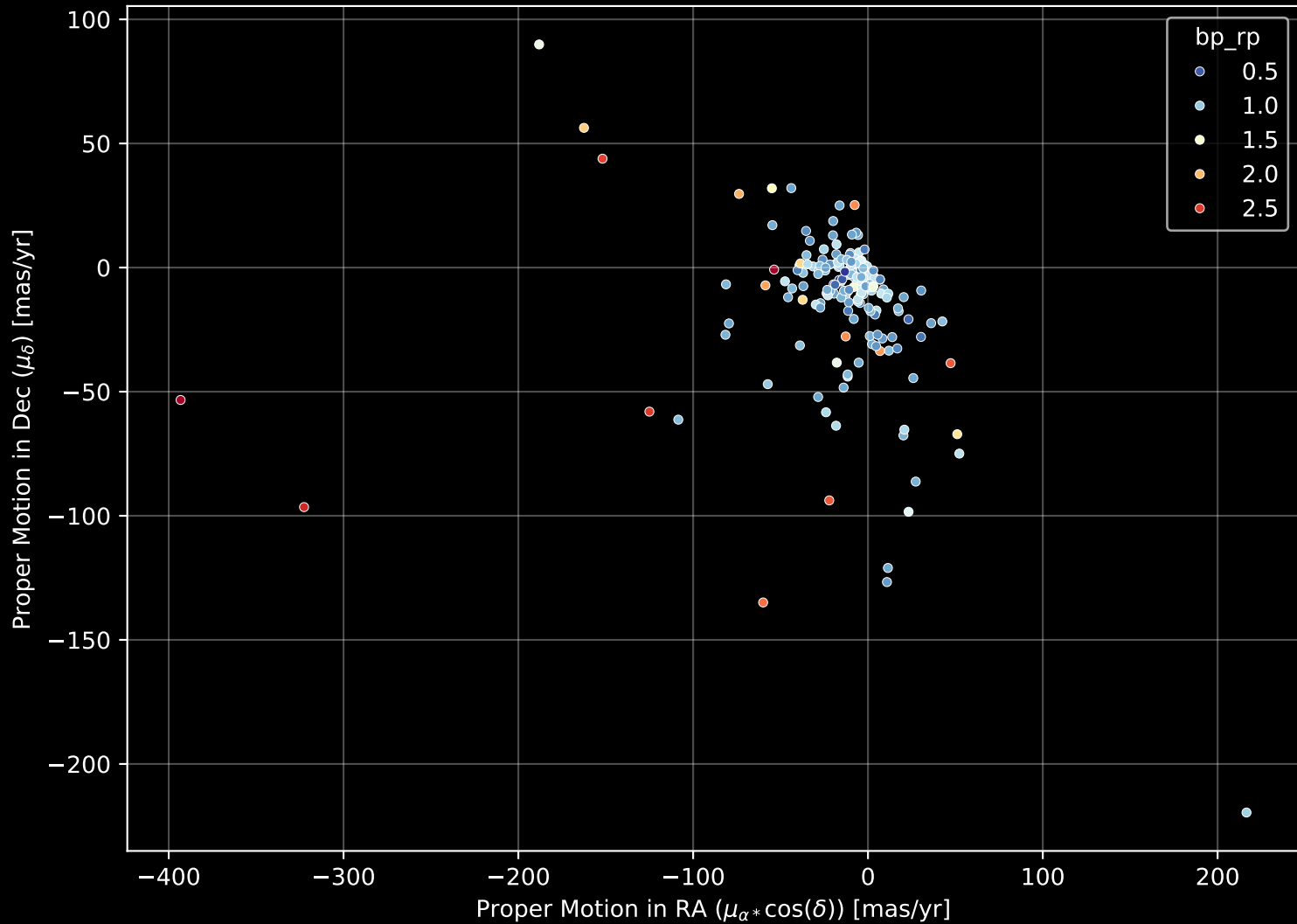
APOGEE DR17 Field: [232+42_MGA] Proper Motion Diagram (n= 184)
