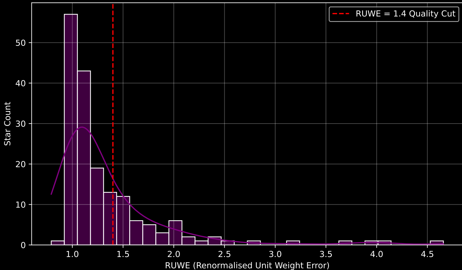
GAPOGEE DR17 Field [232+42_MGA] RUWE Distribution (n= 177)
