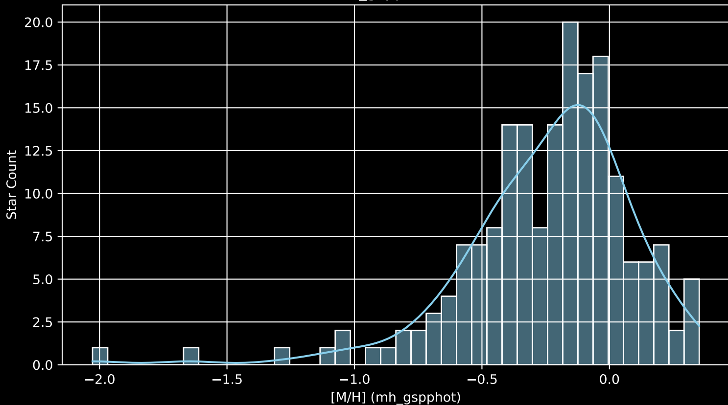
APOGEE DR17 Field: [232+42_MGA [M/H] (mh_gspphot) (n= 183)
