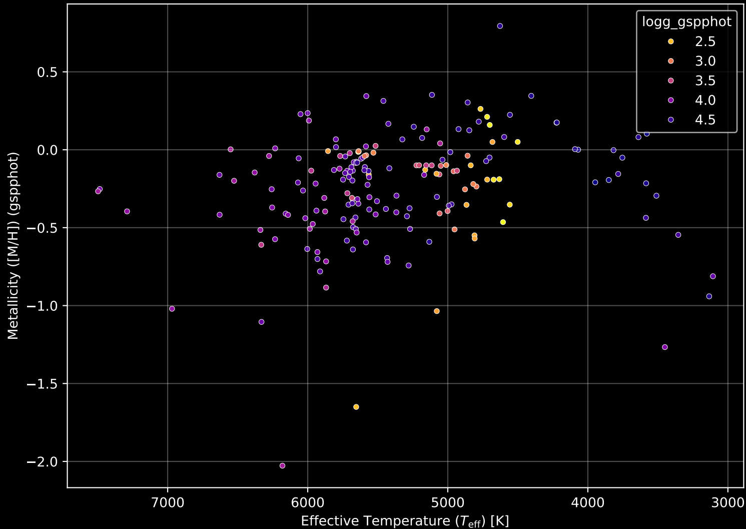
APOGEE DR17 Field: [232+42_MGA] Stellar Population Parameters (n= 184)
