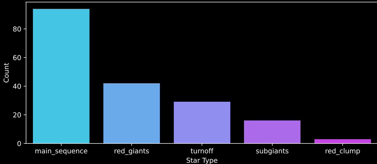
APOGEE DR17 Field: [232+42_MGA] Count plot of Star Type
